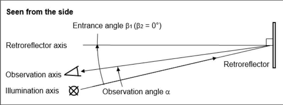
Figure C1: Geometry in a single plane.
