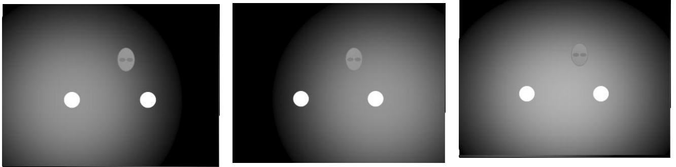
Figure D.2: Retroreflected illumination around the two headlamps (left and middle) and the total illumination (right).
