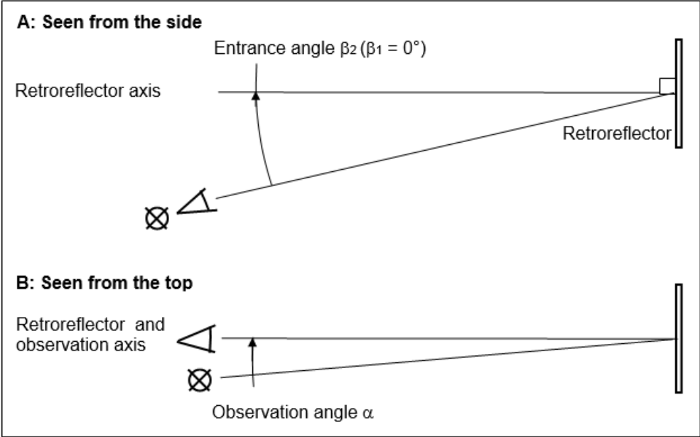
Figure C2: Geometry in two planes.
