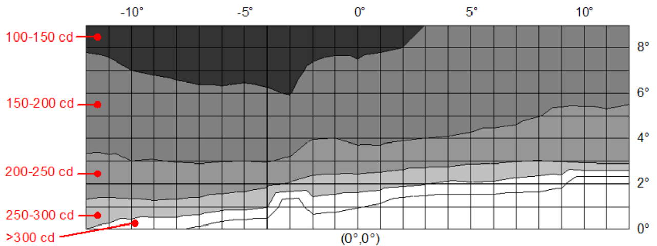
Figure D.3: A typical light distribution of low beam headlamps.
